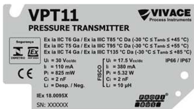
Figura 5.2 – Plaqueta Ex ia do VPT11-P.
